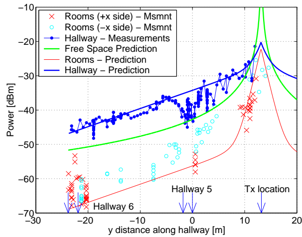
Fig. 6. Median power in Hallway 1 and adjacent rooms. The hallway data are at points 0.5 m or more from both walls. The room data are at points between 1 m and 5 m from one of the hallway walls. The geometry is shown in Figure 2. Model parameters are \epsilon = 3 , \sigma = 0.035 S/m, D = 2 m, s^2 = 0.2 m 2 and hallway width is 1.8 m. The power distribution at the transmitter is a TE narrow source in the middle of the hallway.
