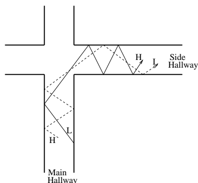
Fig. 13. A hallway corner model. The solid line represents a low order mode of the main hallway coupled into a high order mode of the side hallway. The dashed line represents a high order mode of the main hallway coupled into a low order mode of the side hallway.
