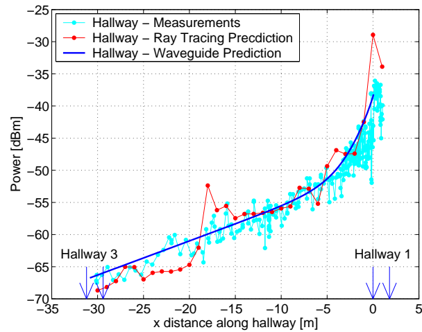
Fig. 14. Median power in Hallway 5, with predictions of the waveguide model and the WiSE ray tracing tool. The geometry is shown in Figure 2.
