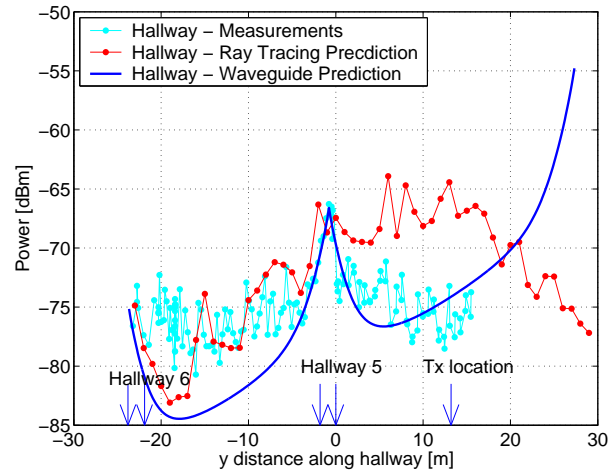
Fig. 17. Median power in Hallway 3, with predictions of the waveguide model and the WiSE ray tracing tool. The geometry is shown in Figure 2.
