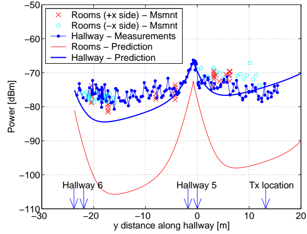
Fig. 10. Median power in Hallway 3 and adjacent rooms. The hallway data are at points 0.5 m or more from both walls. The room data are at points between 1 m and 5 m from one of the hallway walls. The geometry is shown in Figure 2. Model parameters are \epsilon = 3 , \sigma = 0.035 S/m, D = 2 m, s^2 = 0.2 m 2 and hallway width is 1.8 m. The power distribution at the junction is uniform.
