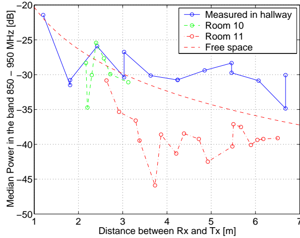
Fig. 3. Power received near the transmitter; The geometry is shown in Figure 2. The free space curve is an estimation based on measurements at close range.
