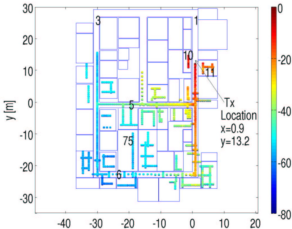
Fig. 2. Locations of the transmitter and receiver in the Packard basement, with median power level at each receiver location [dB]. The single digit numbers indicate hallways and the two-digit numbers indicate rooms in the building. The lines indicate the inner boundary of the hallway and room walls. Details of the walls and doors were omitted.
