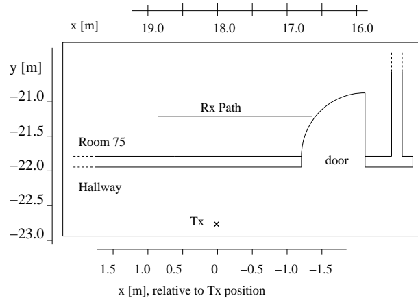
Fig. 5. Geometry of the measurements near room 75.
