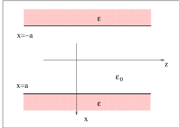
Fig. 11. A smooth slab waveguide
