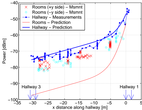
Fig. 9. Median power in Hallway 6 and adjacent rooms. The hallway data are at points 0.5 m or more from both walls. The room data are at points between 1 m and 5 m from one of the hallway walls. The geometry is shown in Figure 2. Model parameters are \epsilon = 3 , \sigma = 0.035 S/m, D = 2 m, s^2 = 0.2 m 2 and hallway width is 1.8 m. The power distribution at the junction is uniform.
