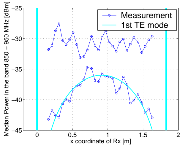
Fig. 7. Power across Hallway 1 (median over band). Top: The receiver is 4.4 m from the transmitter. Bottom: The receiver is 12 m from the transmitter. The vertical lines indicate the inner boundary of the hallway walls.
