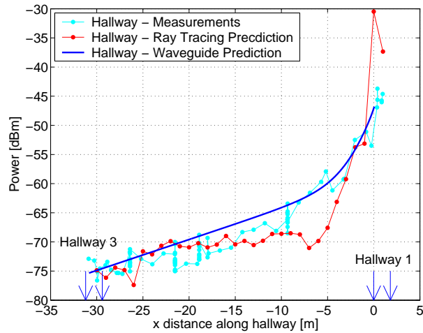
Fig. 15. Median power in Hallway 6, with predictions of the waveguide model and the WiSE ray tracing tool. The geometry is shown in Figure 2.
