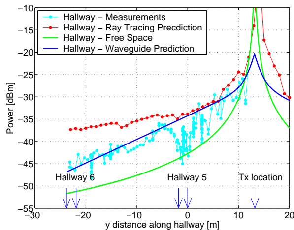
Fig. 16. Median power in Hallway 1, with predictions of three models: the waveguide model, the WiSE ray tracing tool and free space. The geometry is shown in Figure 2.
