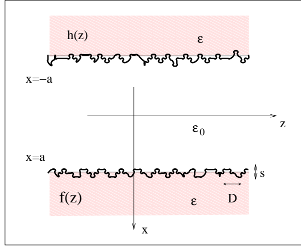
Fig. 12. A rough slab waveguide
