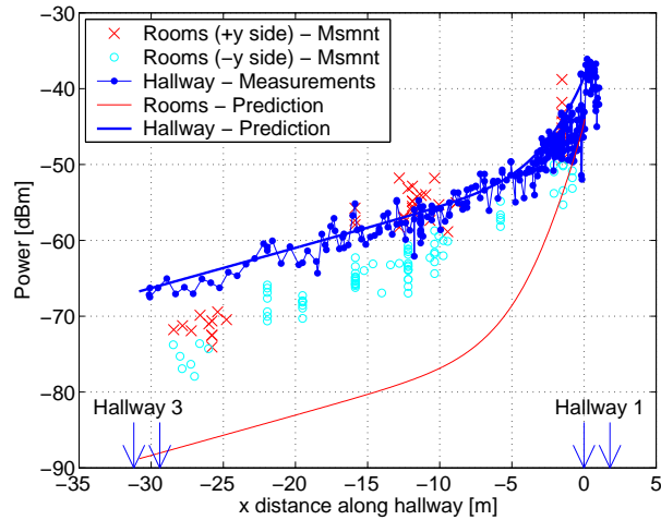
Fig. 8. Median power in Hallway 5 and adjacent rooms. The hallway data are at points 0.5 m or more from both walls. The room data are at points between 1 m and 5 m from one of the hallway walls. The geometry is shown in Figure 2. Model parameters are \epsilon = 3 , \sigma = 0.035 S/m, D = 2 m, s^2 = 0.2 m 2 and hallway width is 1.8 m. The power distribution at the junction is uniform.
