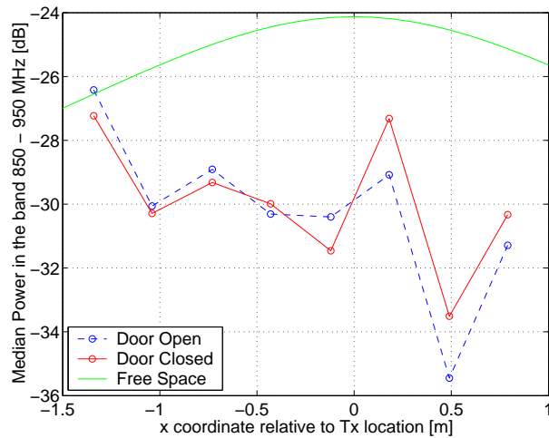
Fig. 4. Power received across a wall; The geometry is shown in Figure 5. The free space curve is an estimation based on measurements at close range.
